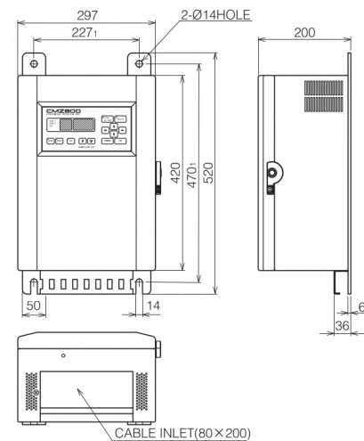
CONTROL BOX (MKC 327)
