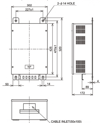
DUAL AC ADAPTER (MKS 071)
