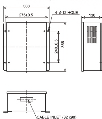
AC ADAPTER (MKS070)
