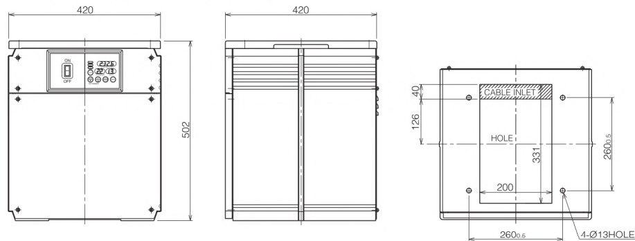
MASTER COMPASS (MKM026)
